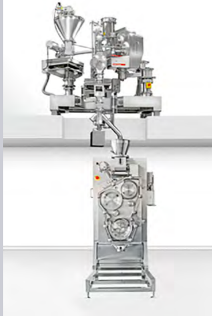
Continuous dry granulation
